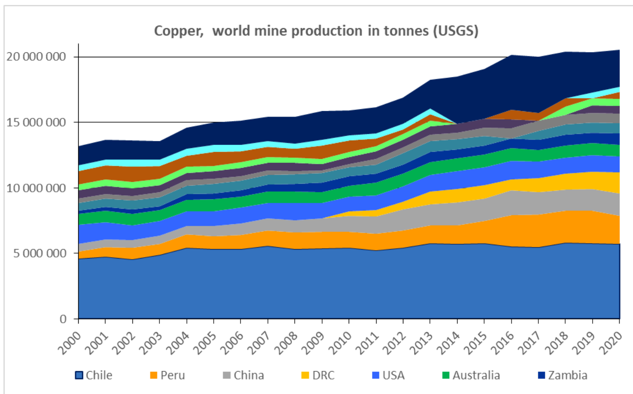
Figure 21: Global mine production of copper in tonnes (USGS Mineral Commodity Summaries 2002 to 2022). When comparing with Figure 1, note that pre-2000 data is not included in the USGS information. The largest producers (as of 2020) shown individually, in decreasing order. DRC = Democratic Republic of Congo, ROW = rest of the world.
